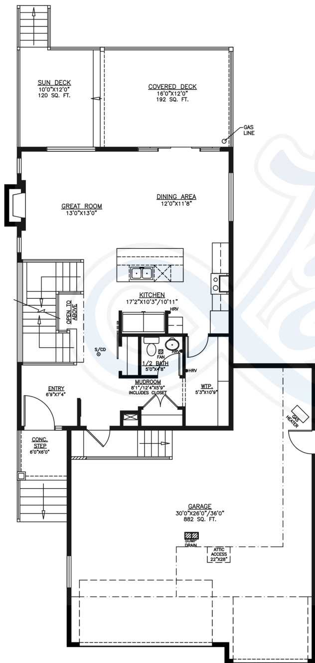
Main Floor 884 SqFt.
